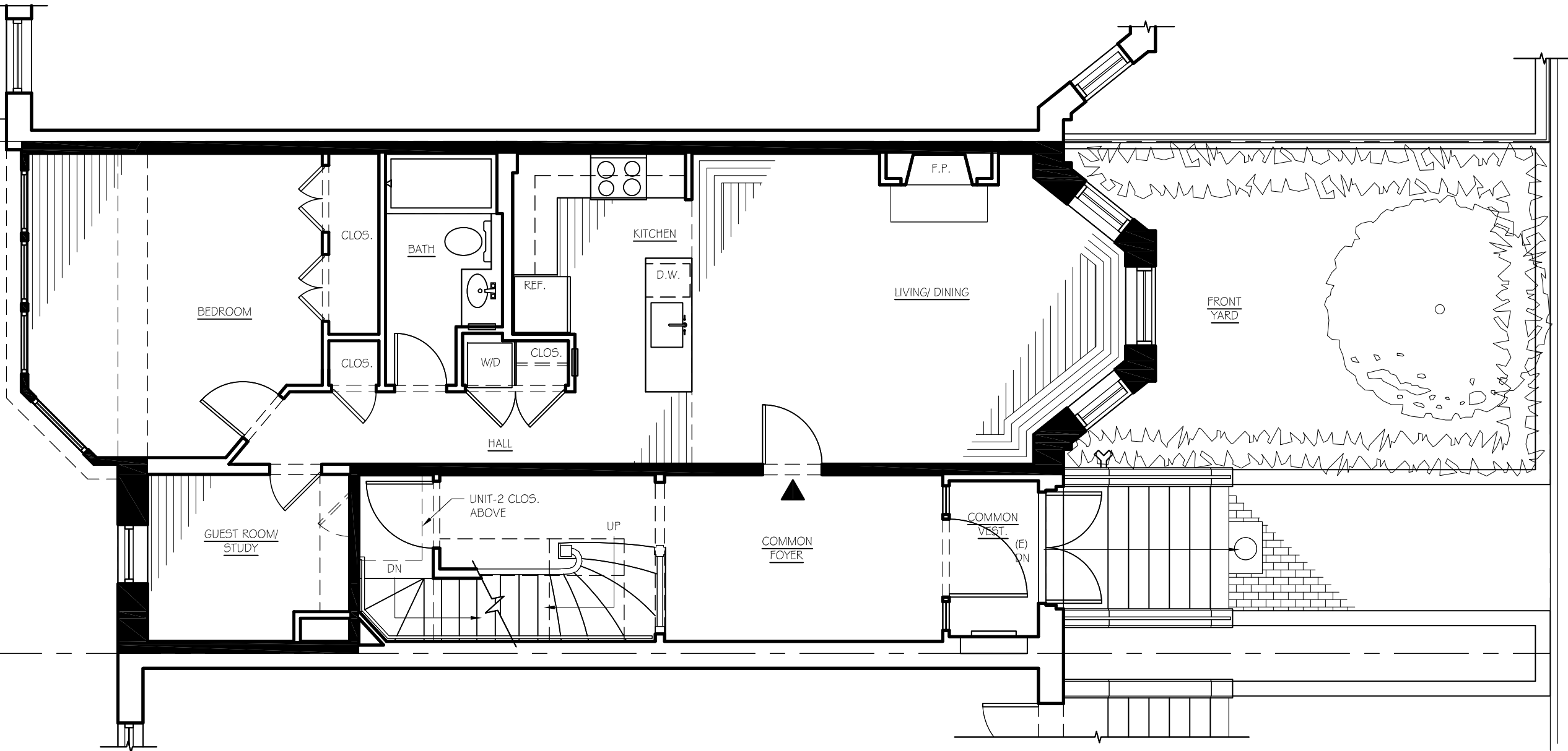
UNIT-2 FLOOR PLAN
